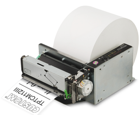
915KV010200300 PRINTER TPTCM112III CUTTER AND NOTCH
